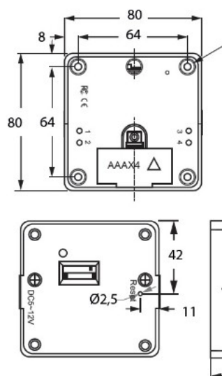
Lock body installation
